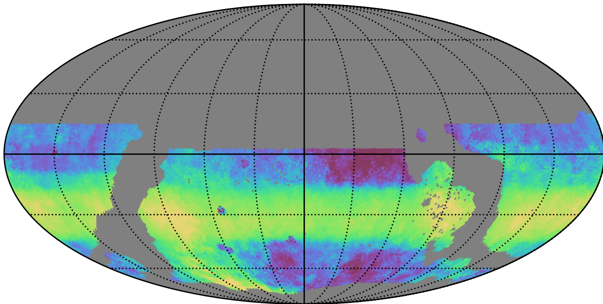
weather_cloudso1v3.4_10yrs WFD y band: Median HA
