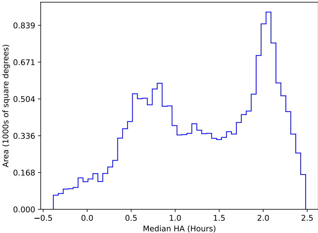
weather_cloudso1v3.4_10yrs WFD y band: Median HA
