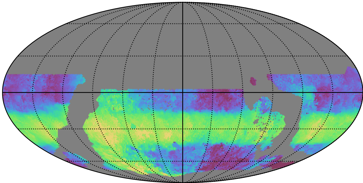
weather_cloudso1v3.4_10yrs WFD u band: Median HA
