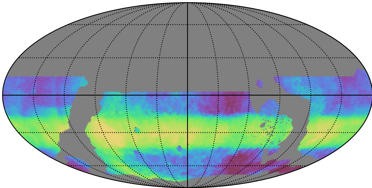
weather_cloudso1v3.4_10yrs WFD r band: Median HA
