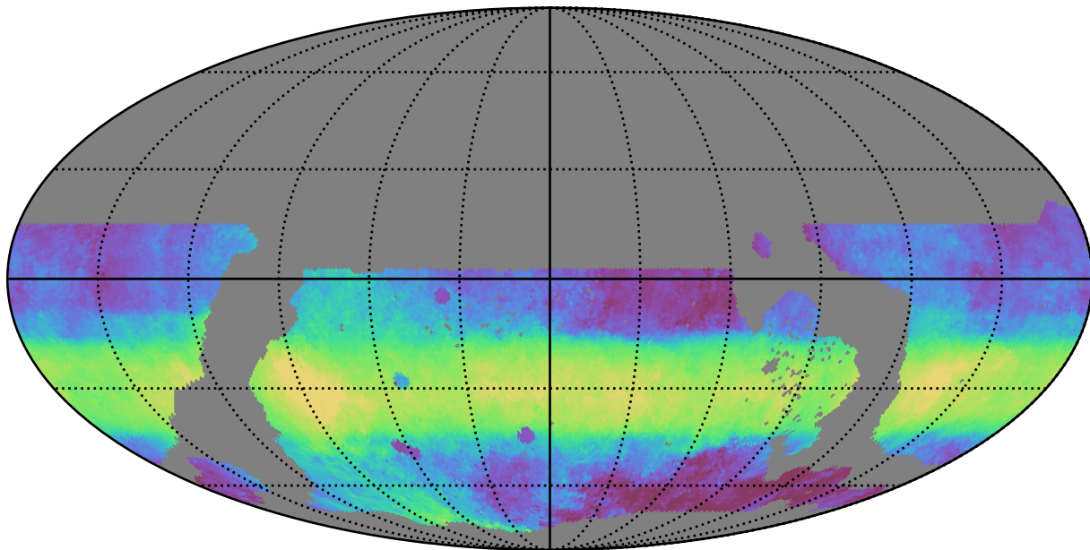
weather_cloudso1v3.4_10yrs WFD i band: Median HA
