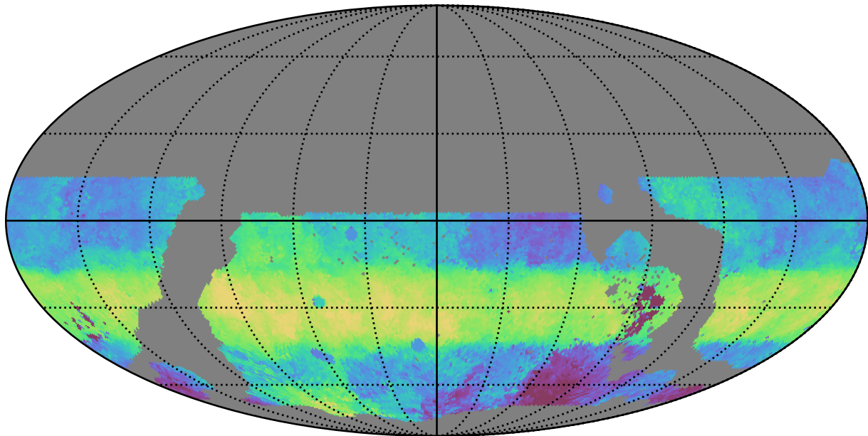
weather_cloudso1v3.4_10yrs WFD g band: Median HA
