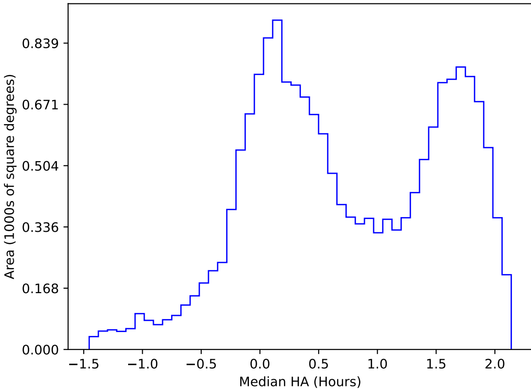
weather_cloudso1v3.4_10yrs WFD g band: Median HA
