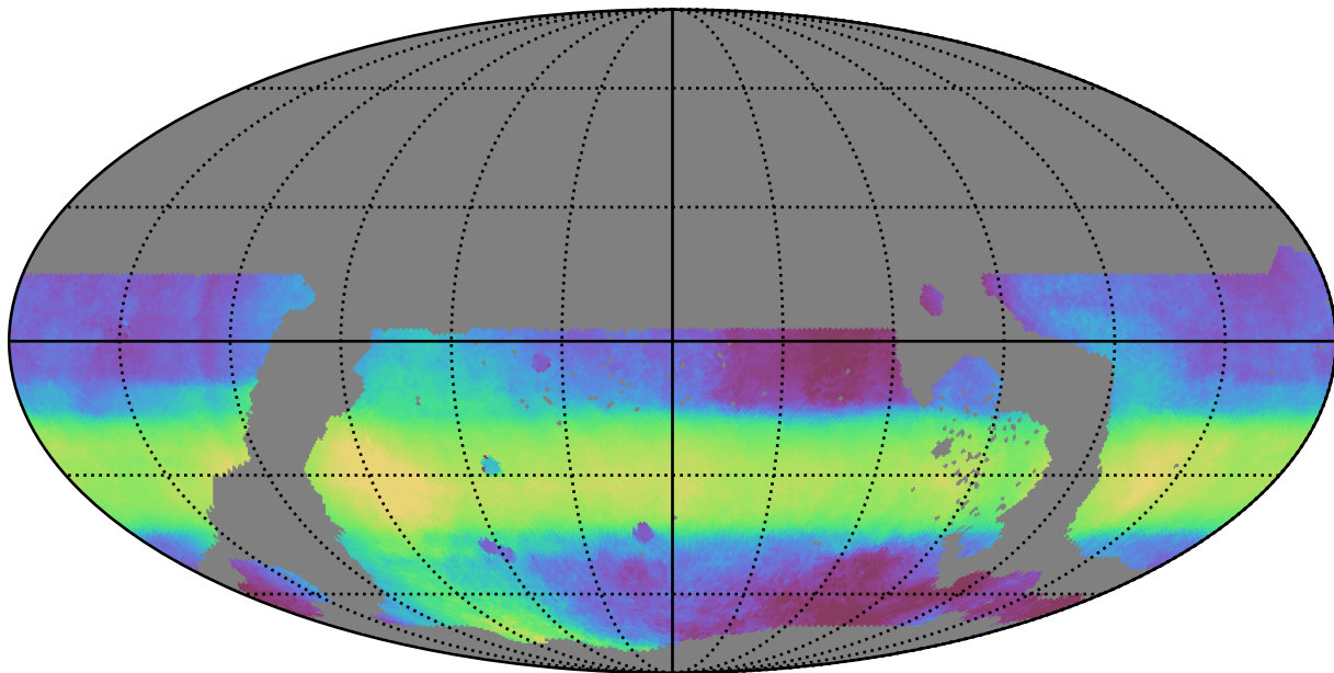
weather_cloudso1v3.4_10yrs WFD all bands: Median HA
