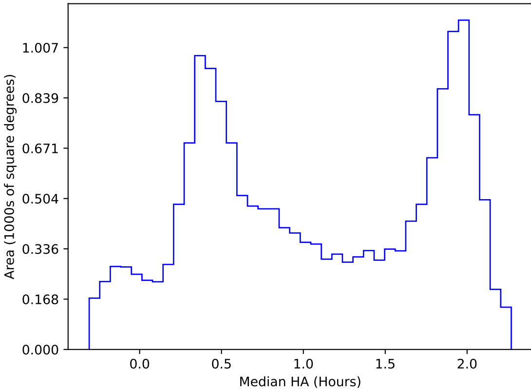
weather_cloudso1v3.4_10yrs WFD all bands: Median HA
