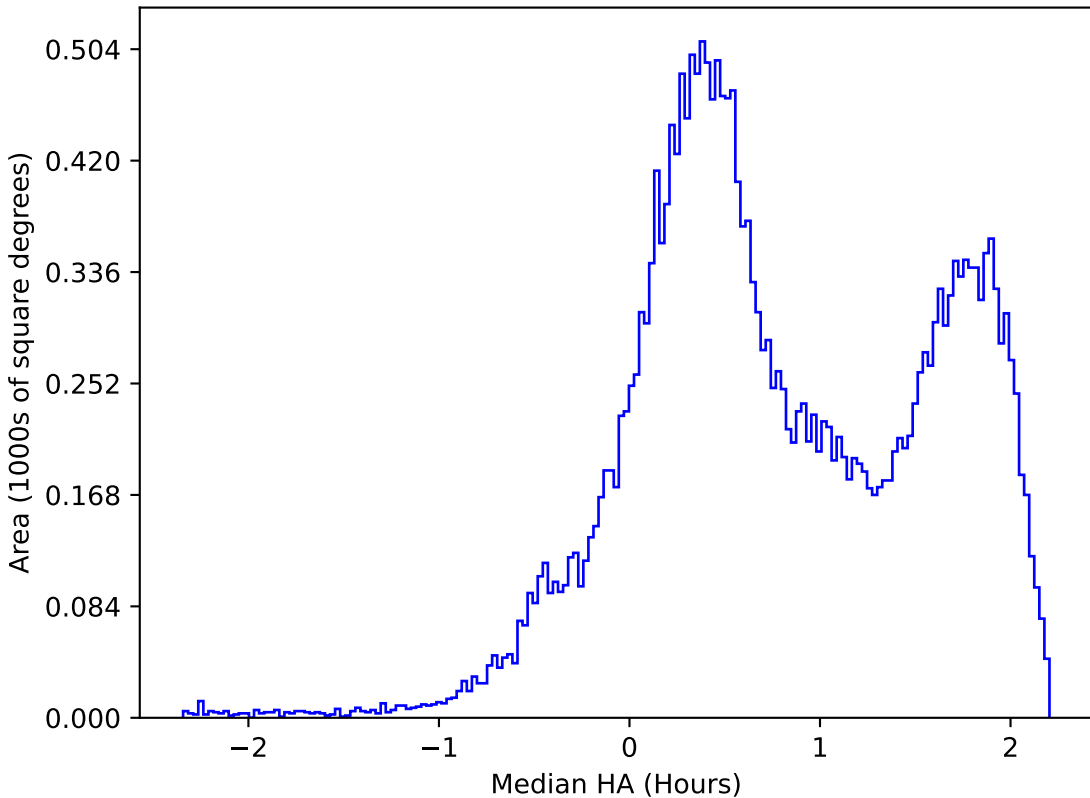
weather_cloudso1v3.4_10yrs All sky r band: Median HA
