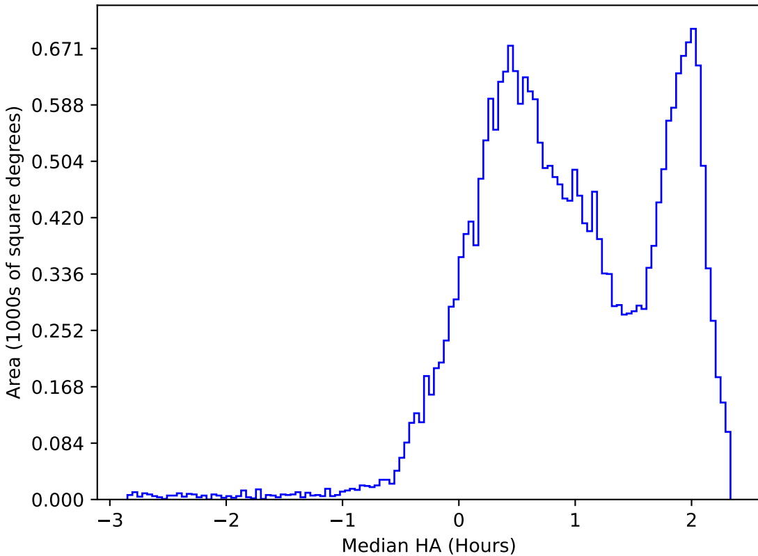
weather_cloudso1v3.4_10yrs All sky i band: Median HA
