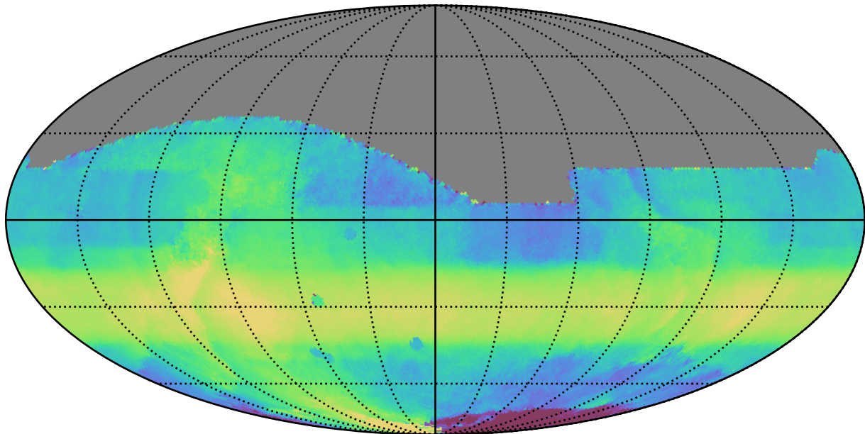
weather_cloudso1v3.4_10yrs All sky all bands: Median HA
