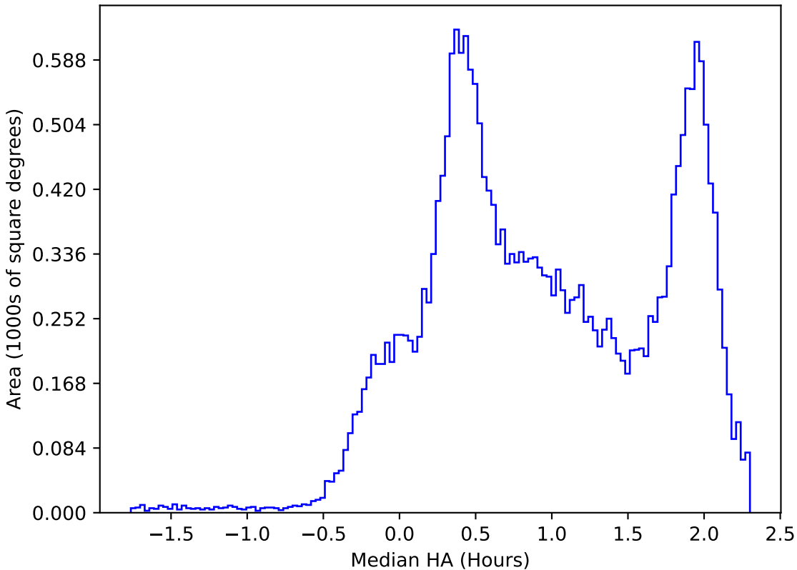
weather_cloudso1v3.4_10yrs All sky all bands: Median HA
