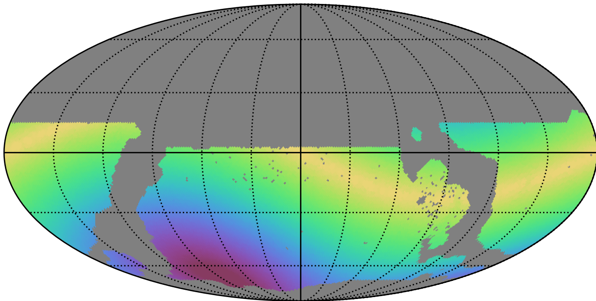
weather_cloudso1v3.4_10yrs WFD z band: Max solarElong
