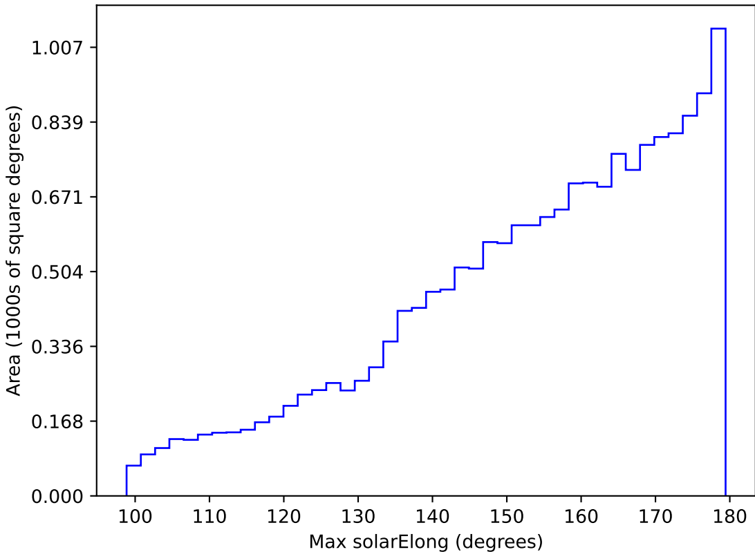
weather_cloudso1v3.4_10yrs WFD z band: Max solarElong
