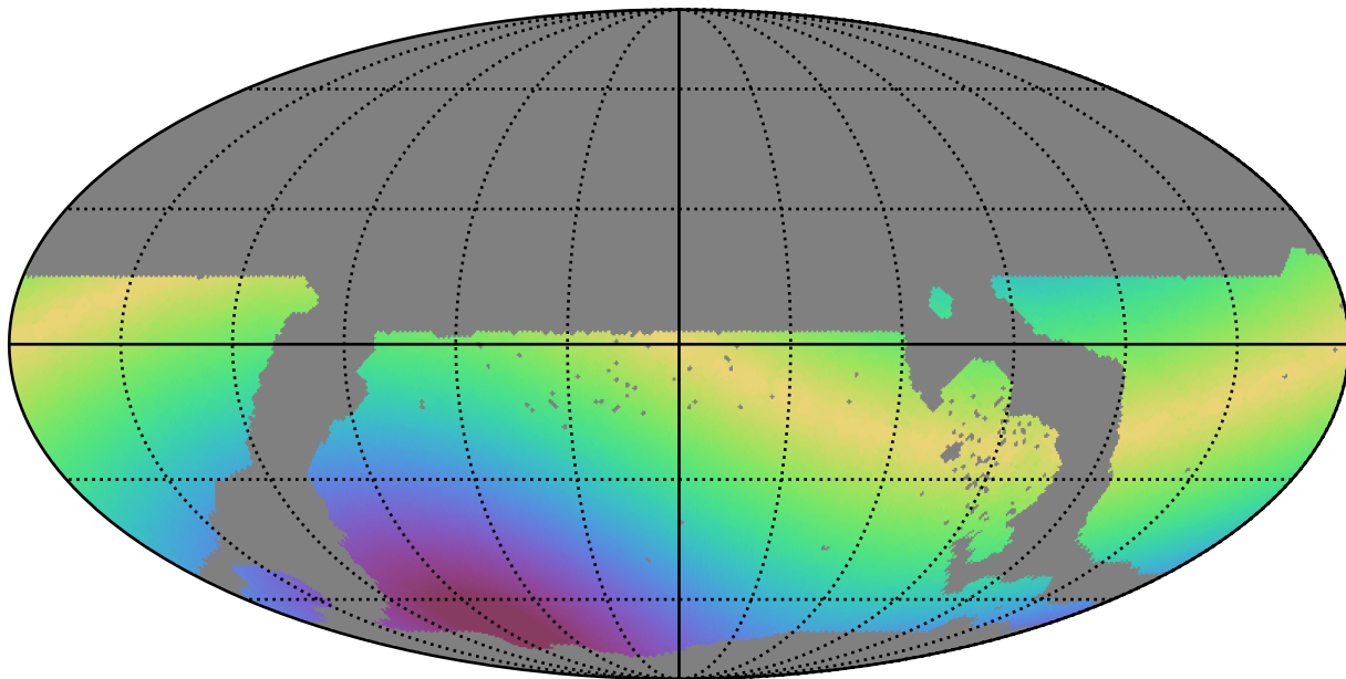
weather_cloudso1v3.4_10yrs WFD y band: Max solarElong
