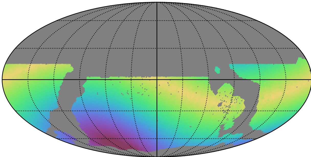
weather_cloudso1v3.4_10yrs WFD u band: Max solarElong
