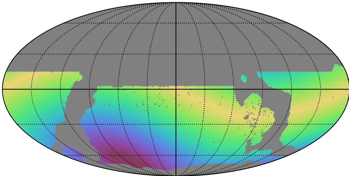
weather_cloudso1v3.4_10yrs WFD i band: Max solarElong
