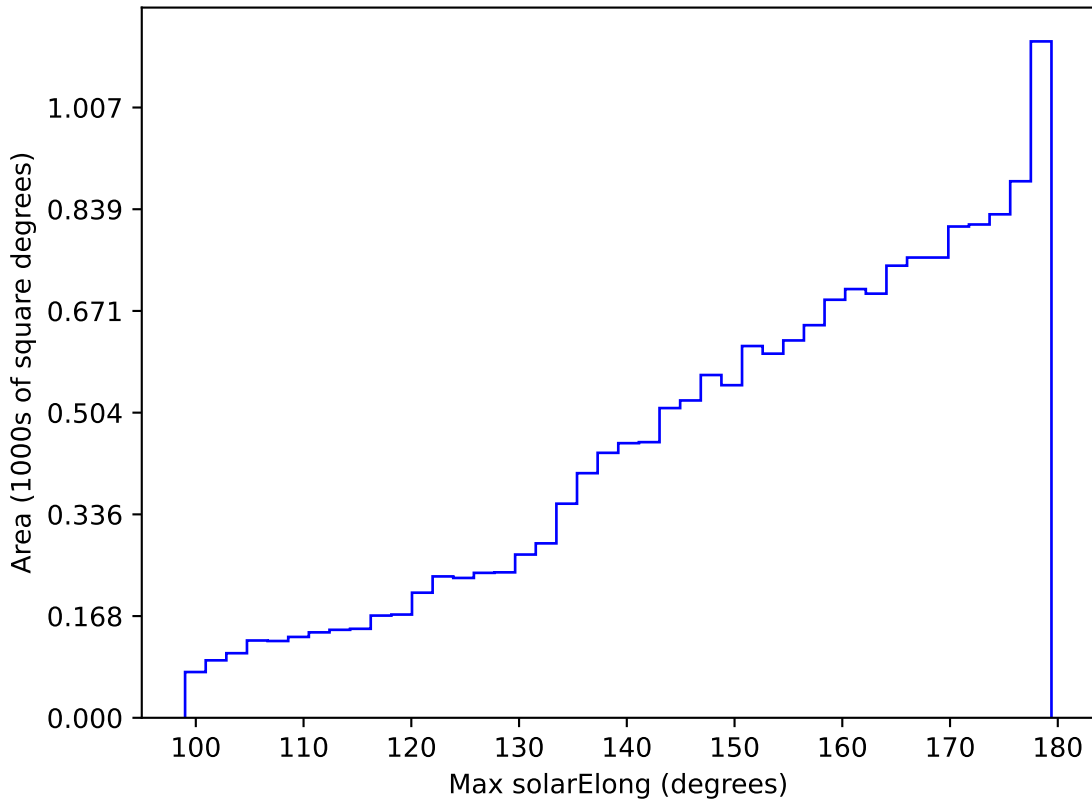
weather_cloudso1v3.4_10yrs WFD i band: Max solarElong
