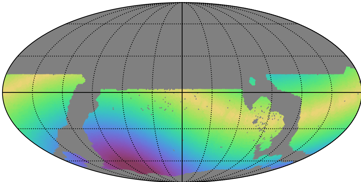
weather_cloudso1v3.4_10yrs WFD g band: Max solarElong
