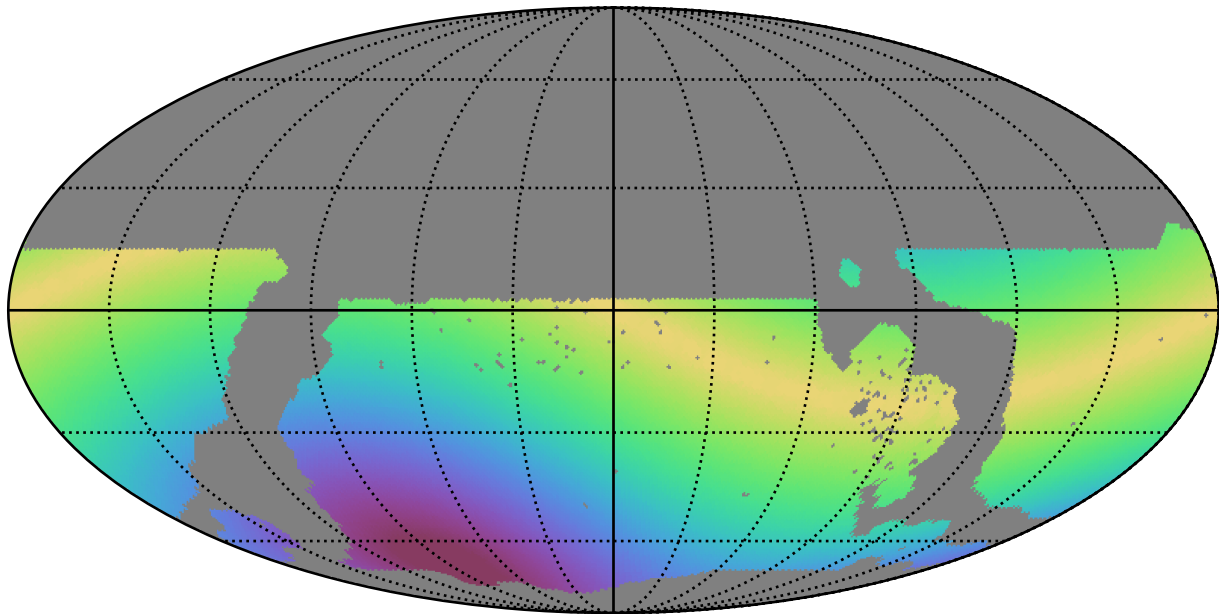
weather_cloudso1v3.4_10yrs WFD all bands: Max solarElong
