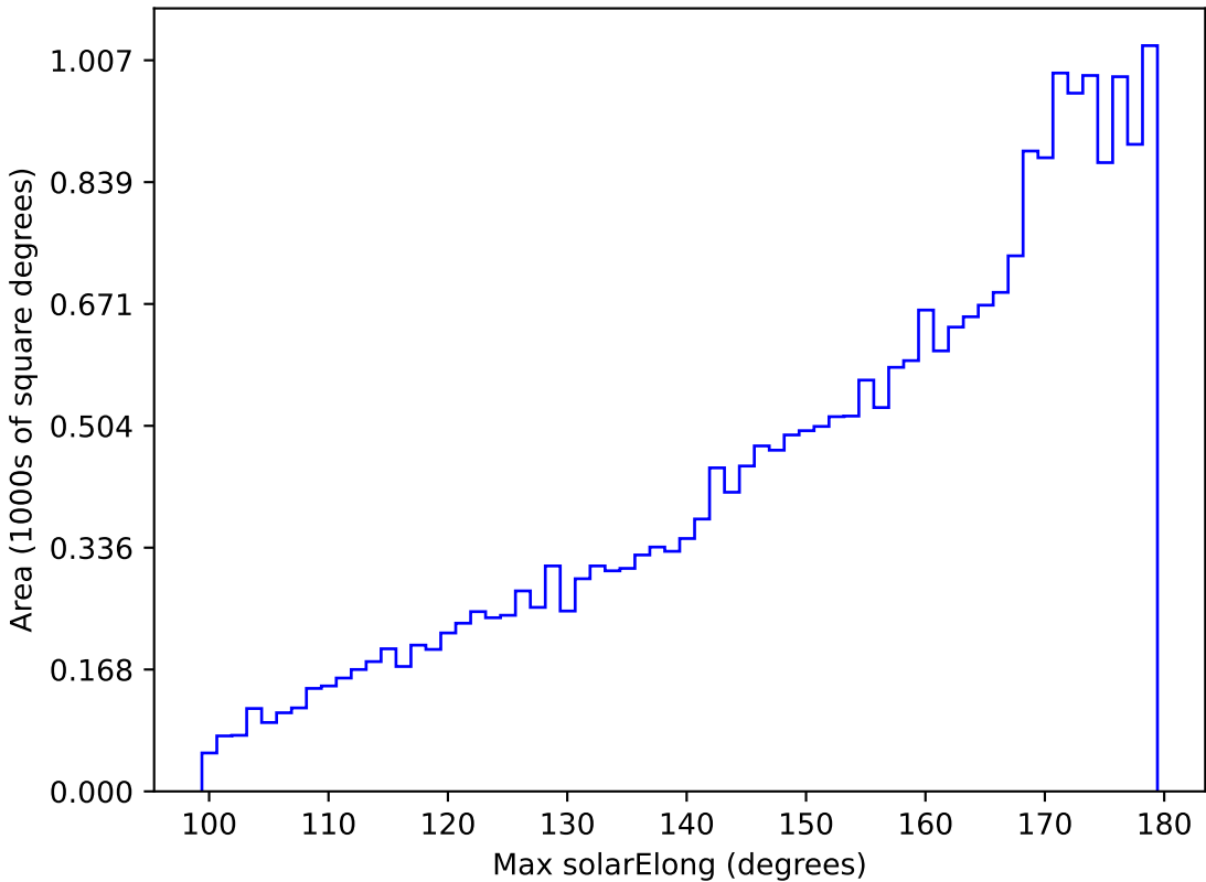
weather_cloudso1v3.4_10yrs All sky z band: Max solarElong
