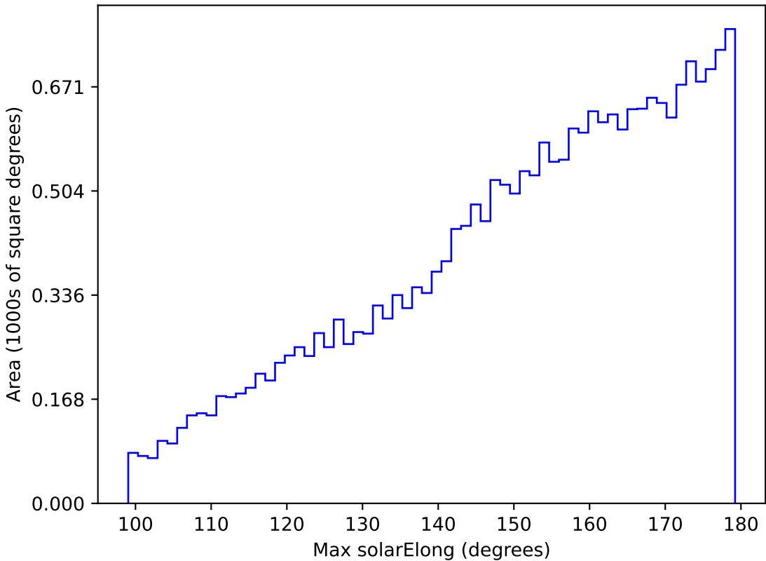
weather_cloudso1v3.4_10yrs All sky y band: Max solarElong
