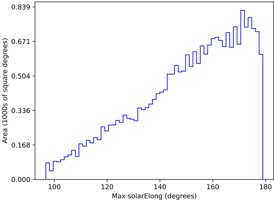
weather_cloudso1v3.4_10yrs All sky u band: Max solarElong
