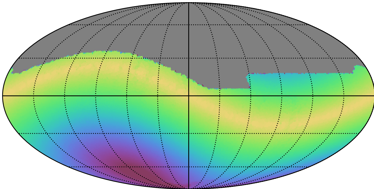
weather_cloudso1v3.4_10yrs All sky r band: Max solarElong
