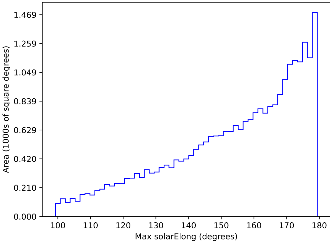
weather_cloudso1v3.4_10yrs All sky r band: Max solarElong
