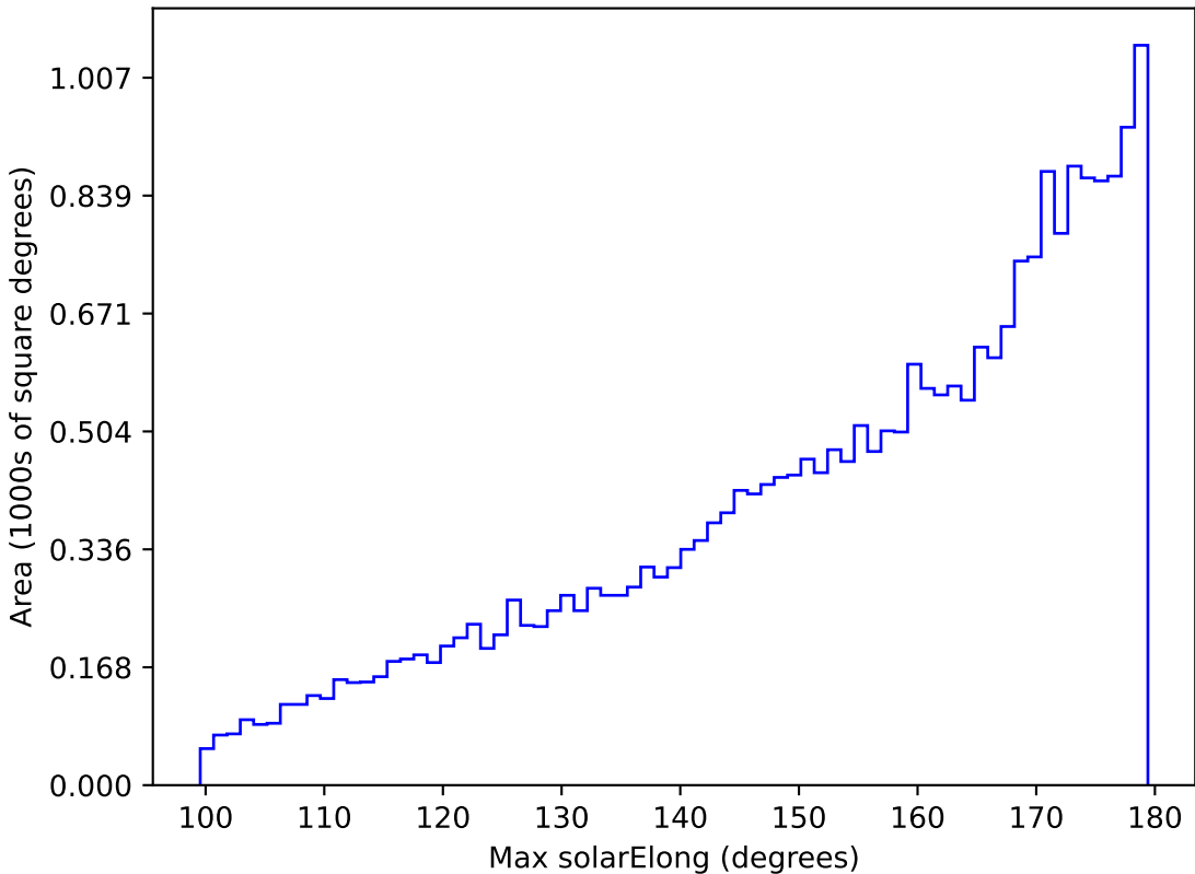
weather_cloudso1v3.4_10yrs All sky i band: Max solarElong
