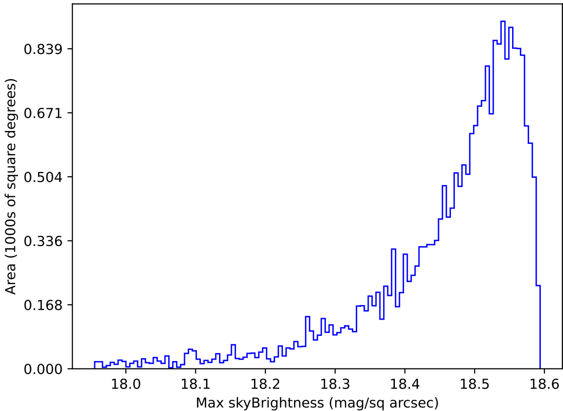
weather_cloudso1v3.4_10yrs Yr 1 y band: Max skyBrightness
