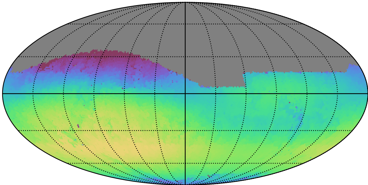
weather_cloudso1v3.4_10yrs Yr 1 r band: Max skyBrightness
