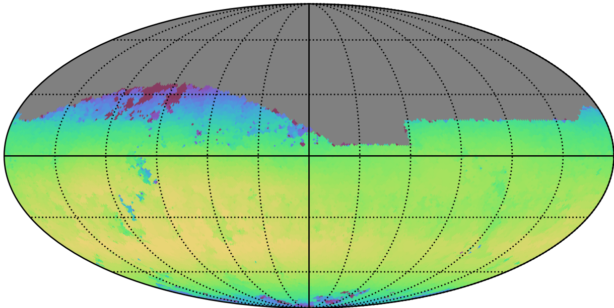
weather_cloudso1v3.4_10yrs Yr 1 i band: Max skyBrightness
