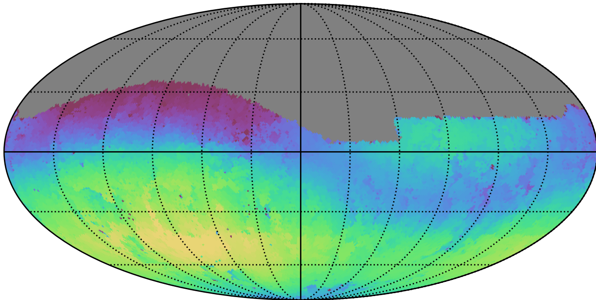
weather_cloudso1v3.4_10yrs Yr 1 g band: Max skyBrightness
