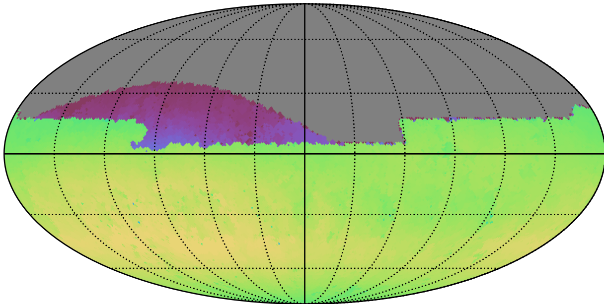
weather_cloudso1v3.4_10yrs Yr1 all bands: Max skyBrightness
