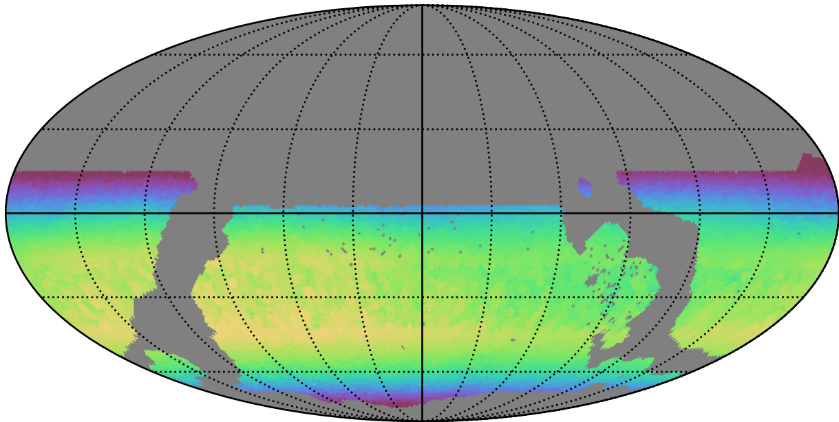
weather_cloudso1v3.4_10yrs WFD z band: Max skyBrightness
