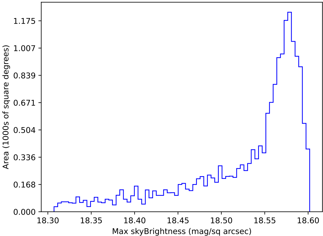
weather_cloudso1v3.4_10yrs WFD y band: Max skyBrightness
