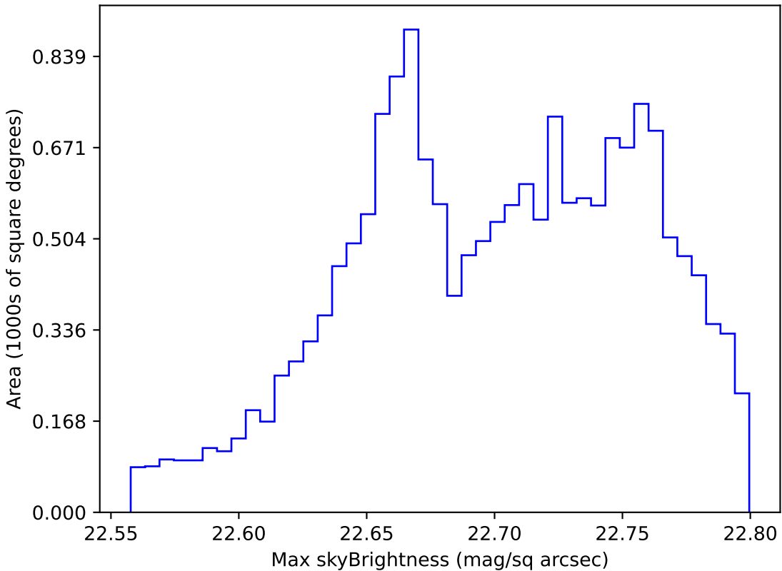
weather_cloudso1v3.4_10yrs WFD u band: Max skyBrightness
