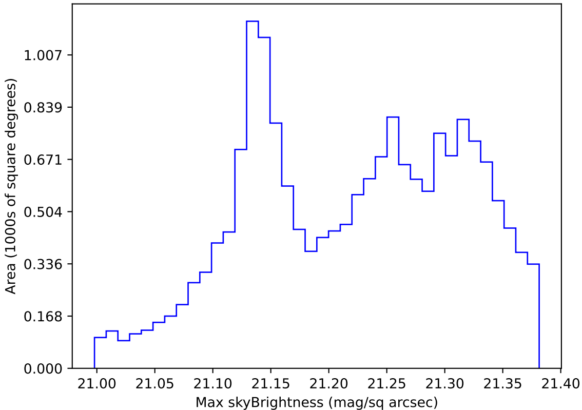
weather_cloudso1v3.4_10yrs WFD r band: Max skyBrightness
