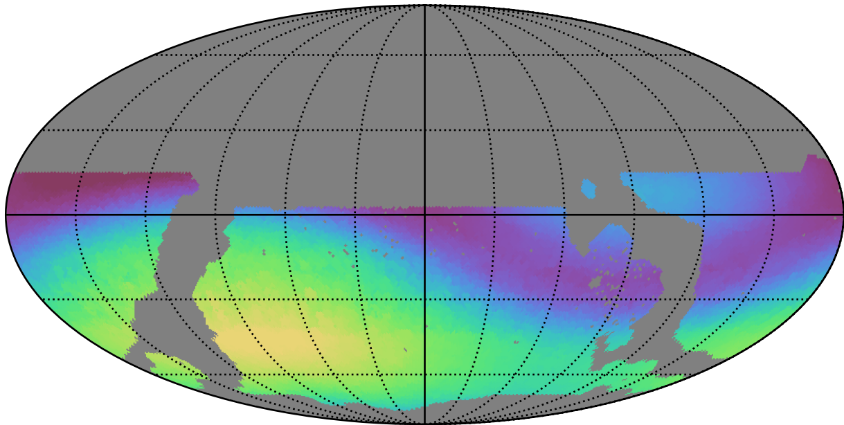
weather_cloudso1v3.4_10yrs WFD g band: Max skyBrightness
