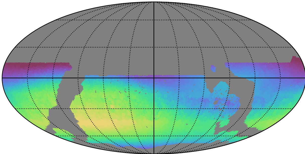
weather_cloudso1v3.4_10yrs WFD all bands: Max skyBrightness
