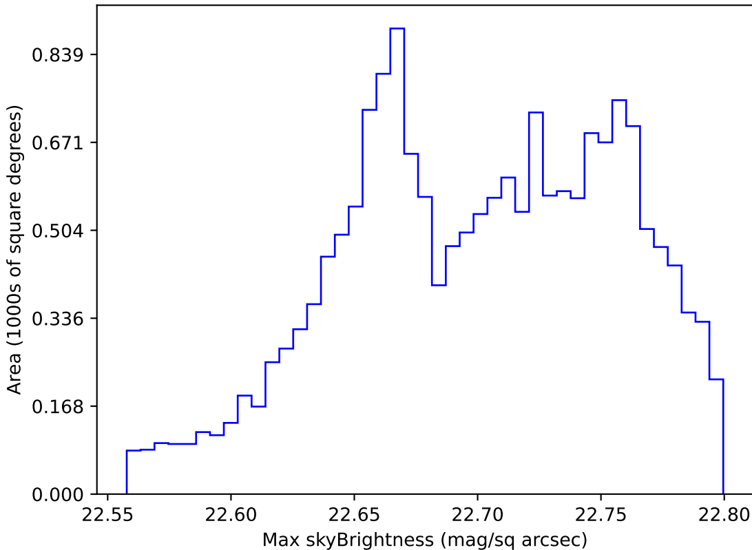
weather_cloudso1v3.4_10yrs WFD all bands: Max skyBrightness
