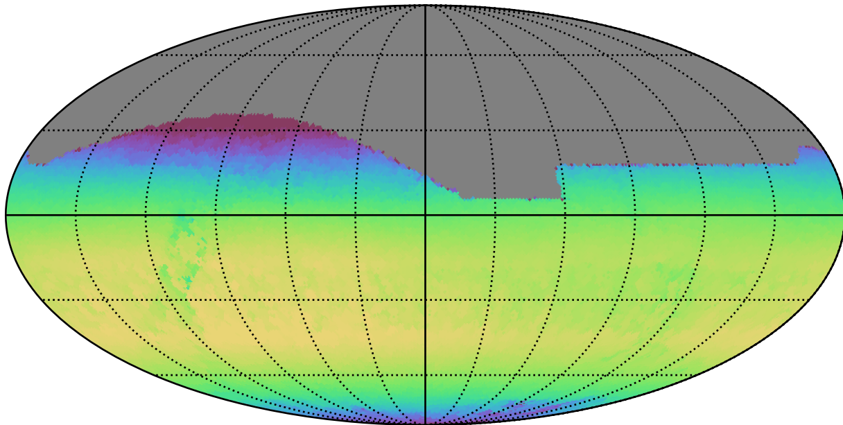
weather_cloudso1v3.4_10yrs All sky z band: Max skyBrightness
