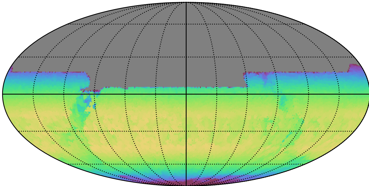
weather_cloudso1v3.4_10yrs All sky y band: Max skyBrightness
