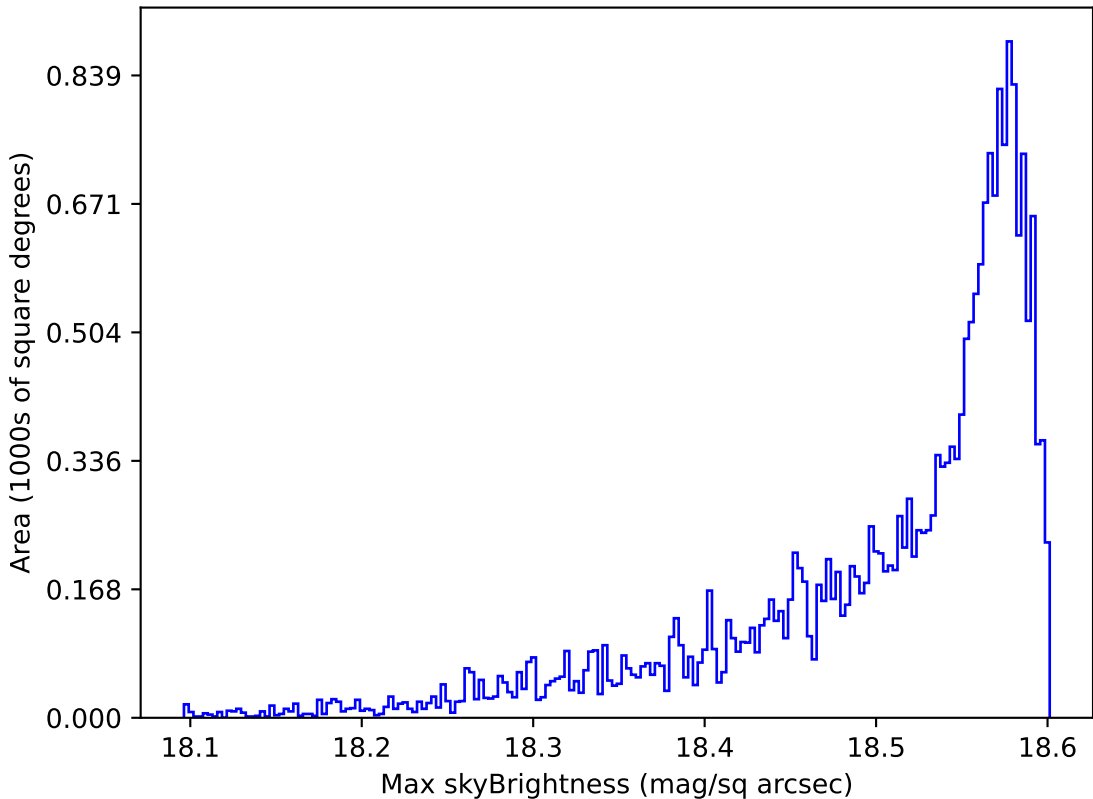
weather_cloudso1v3.4_10yrs All sky y band: Max skyBrightness
