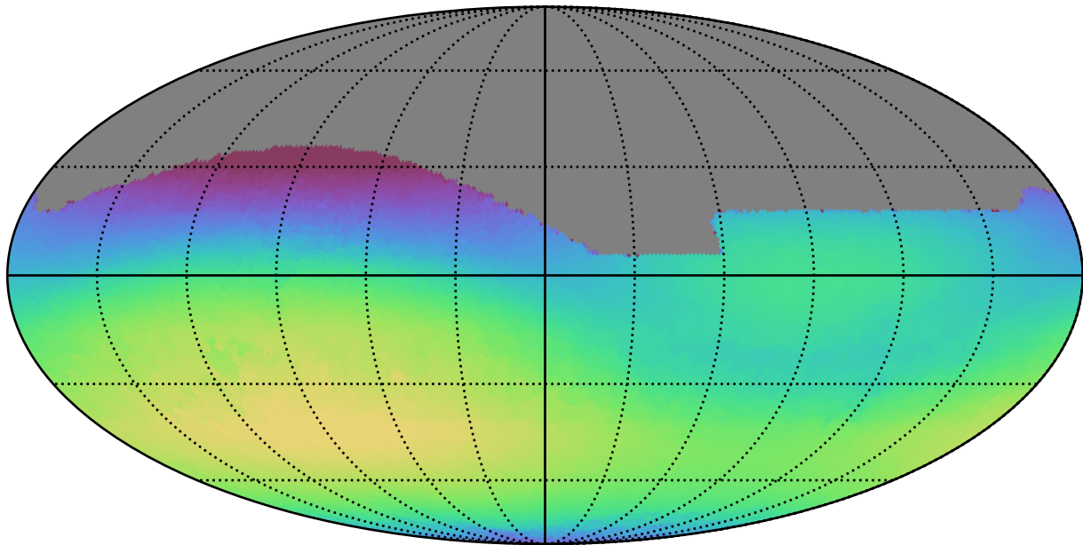
weather_cloudso1v3.4_10yrs All sky r band: Max skyBrightness
