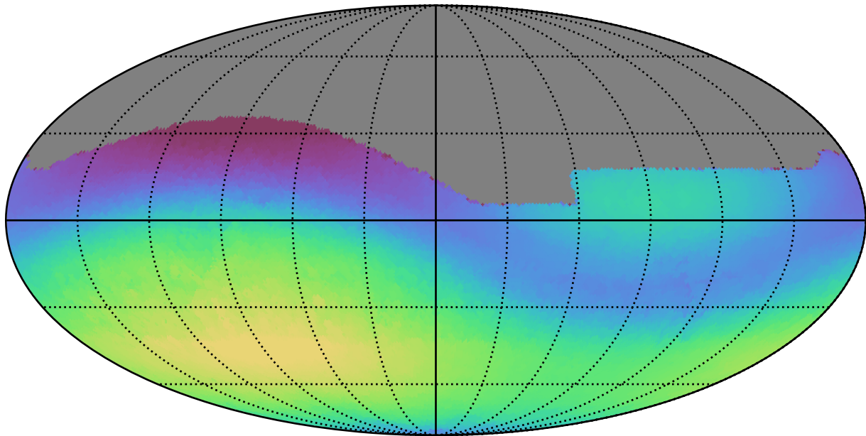
weather_cloudso1v3.4_10yrs All sky g band: Max skyBrightness
