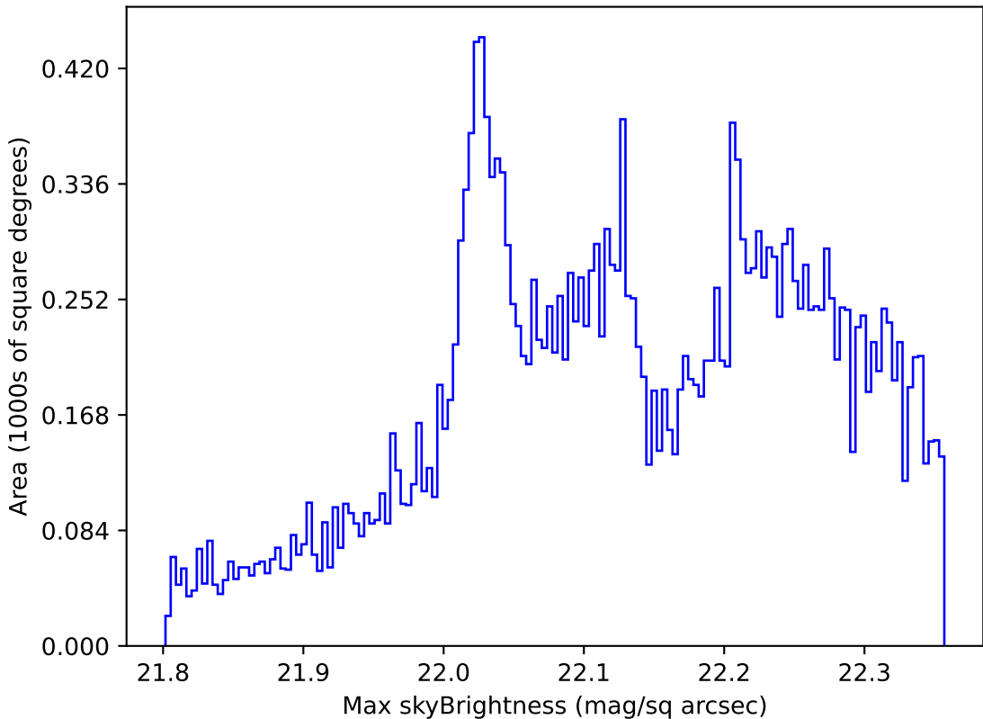
weather_cloudso1v3.4_10yrs All sky g band: Max skyBrightness
