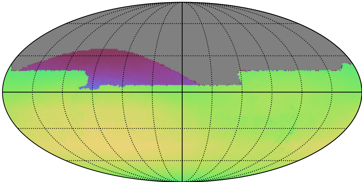
weather_cloudso1v3.4_10yrs All sky all bands: Max skyBrightness
