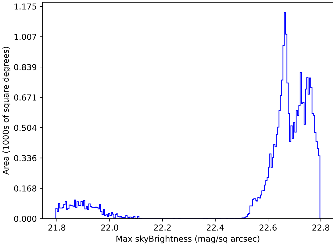
weather_cloudso1v3.4_10yrs All sky all bands: Max skyBrightness
