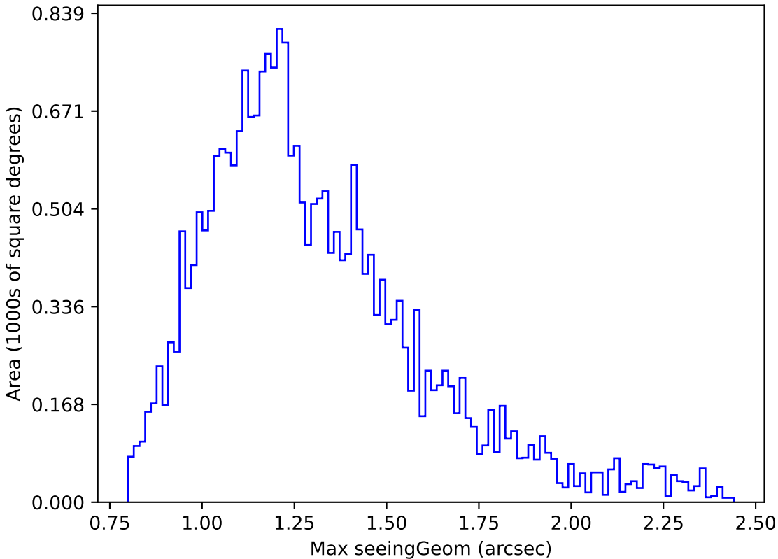
weather_cloudso1v3.4_10yrs Yr 1 z band: Max seeingGeom
