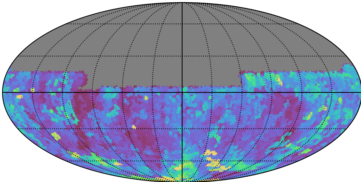
weather_cloudso1v3.4_10yrs Yr 1 y band: Max seeingGeom
