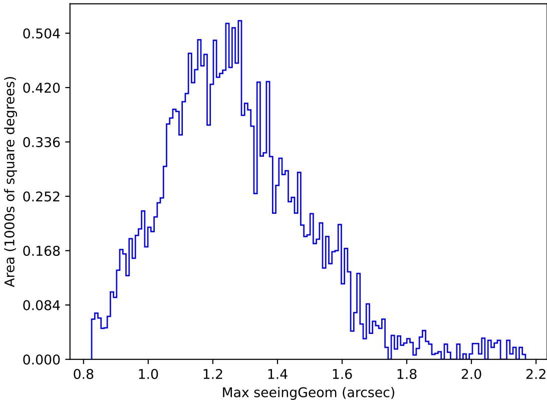
weather_cloudso1v3.4_10yrs Yr 1 y band: Max seeingGeom
